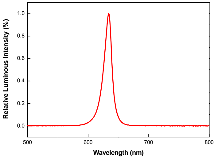
Relative Spectral Distribution, I_F=700\text{mA} , T_{\text{Ambient}}=25^\circ\text{C}
