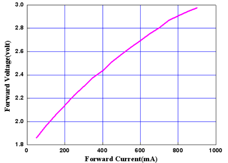
Forward Voltage vs Forward Current, T_{\text{Ambient}}=25^\circ\text{C}
