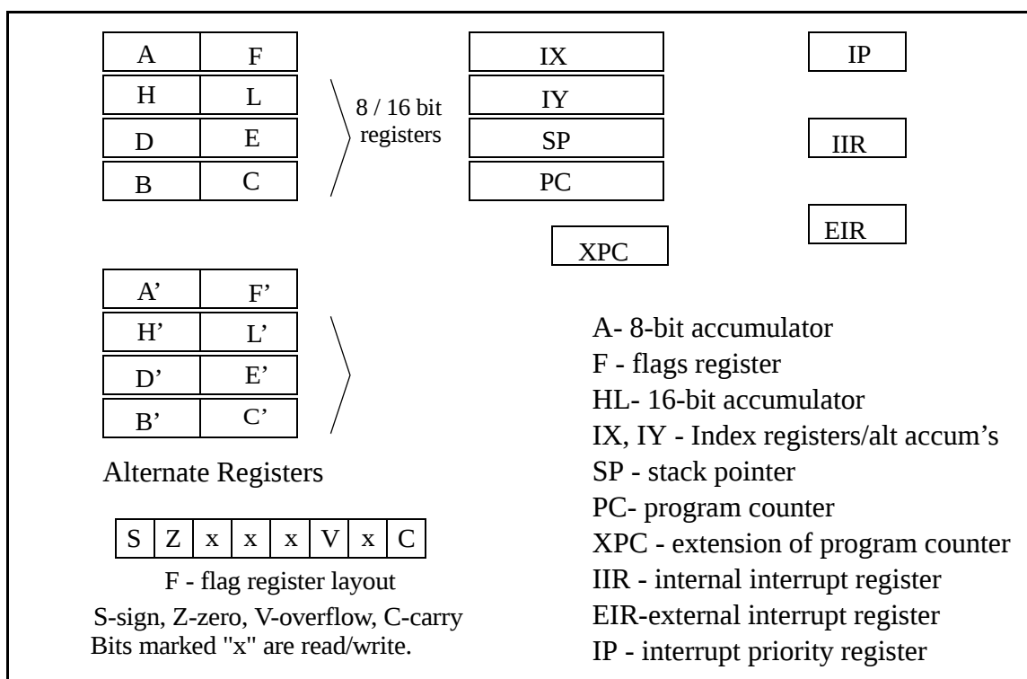
Figure 9. Rabbit Registers
