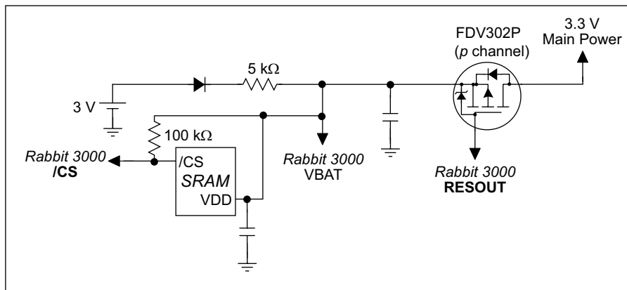
Figure 16. Battery-Backup Circuit
