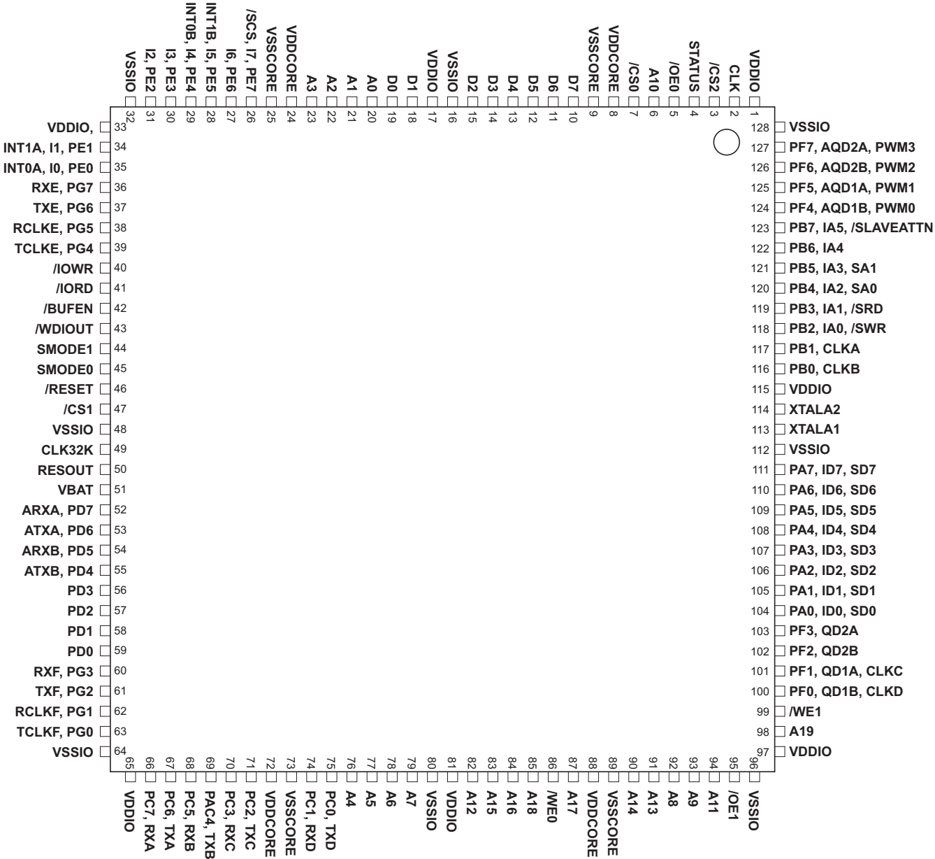
Figure 4. Package Outline and Pin Assignments
