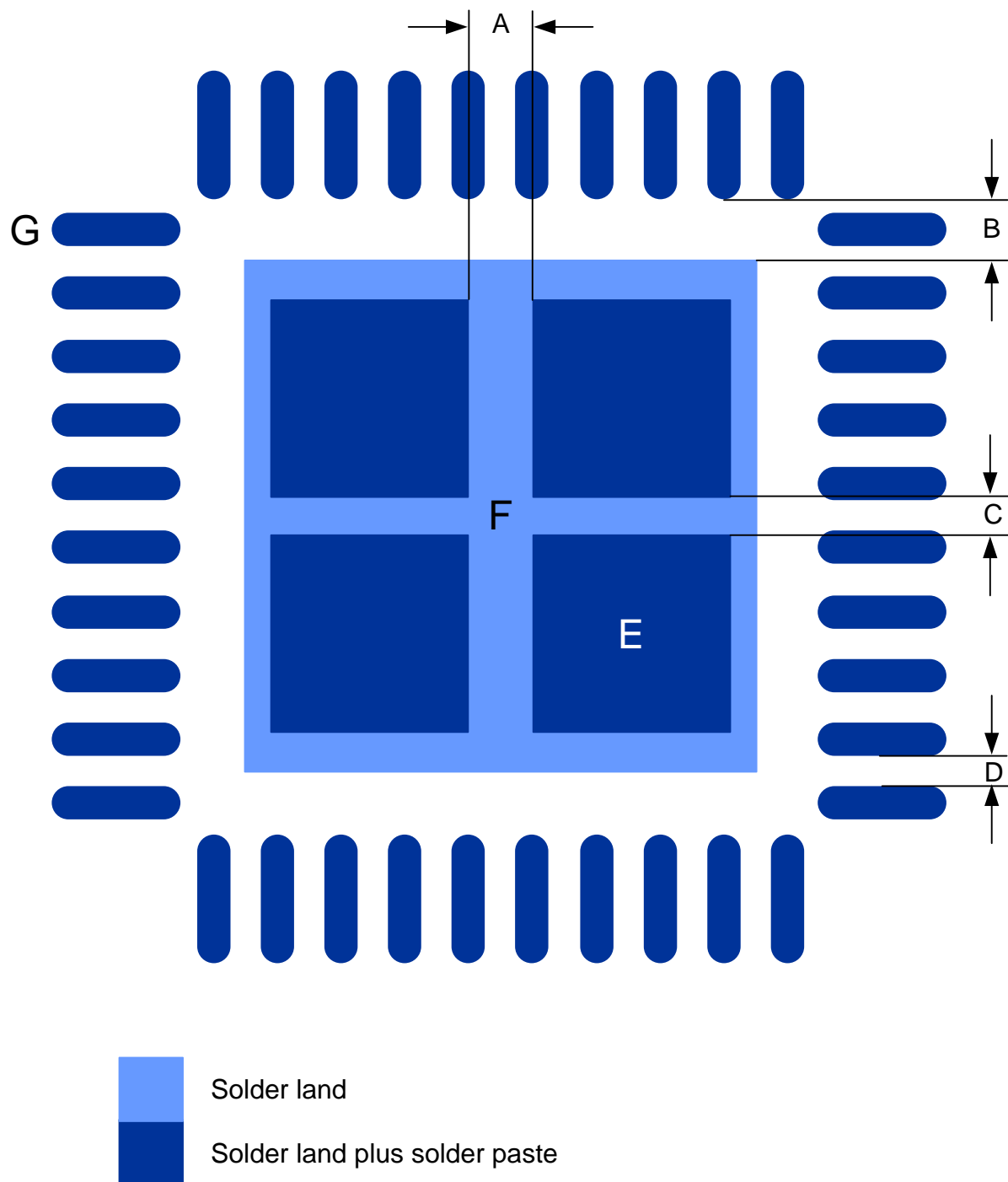
Figure 46: PCB Decal
